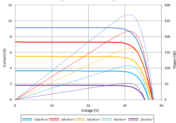
Current-Voltage & Power-Voltage Curve (270)
